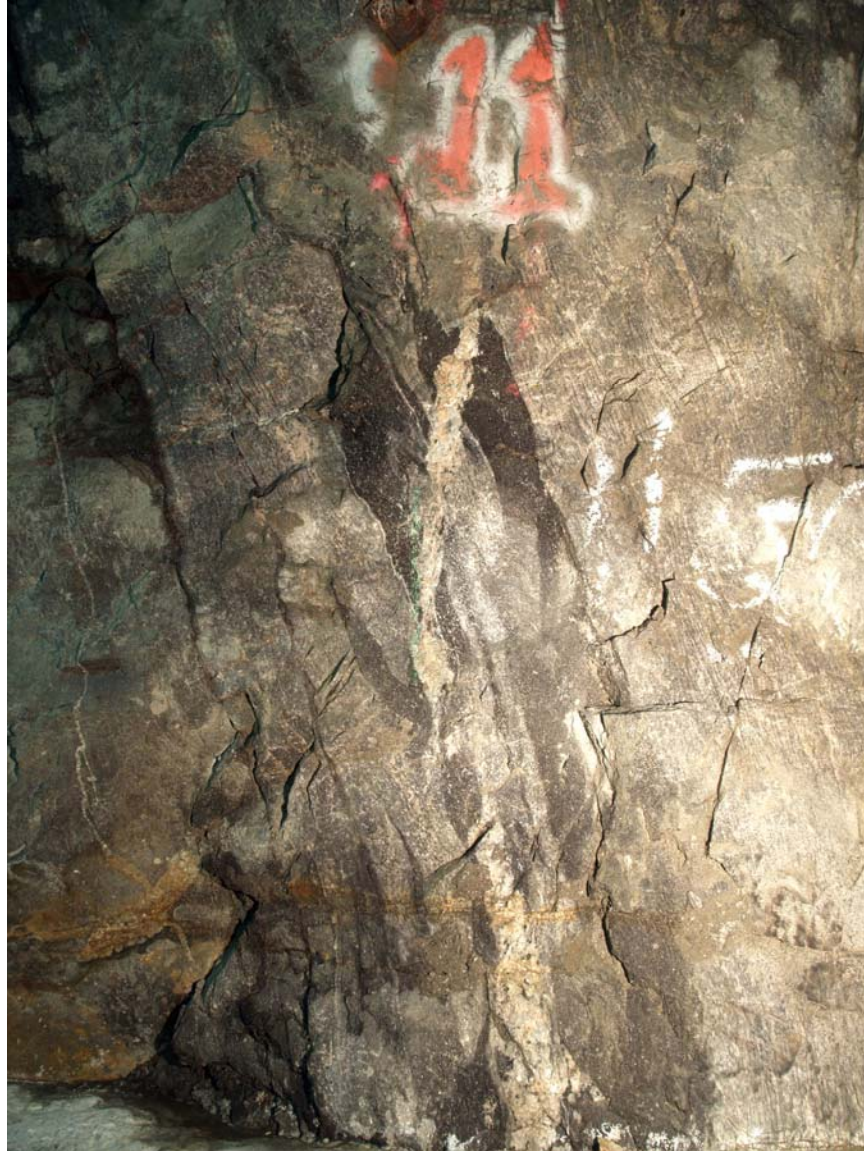
Figure 9 - Diffuse xenoliths of Fordham mafic gneiss flattened into foliation of Yonkers Gneiss near contact zone. Note late pegmatite dike cutting across the xenolith-Yonkers boundaries. Station 5+65, north wall raw water tunnel, Croton Water Treatment Plant, Bronx, New York (Digital image by C. Merguerian).
